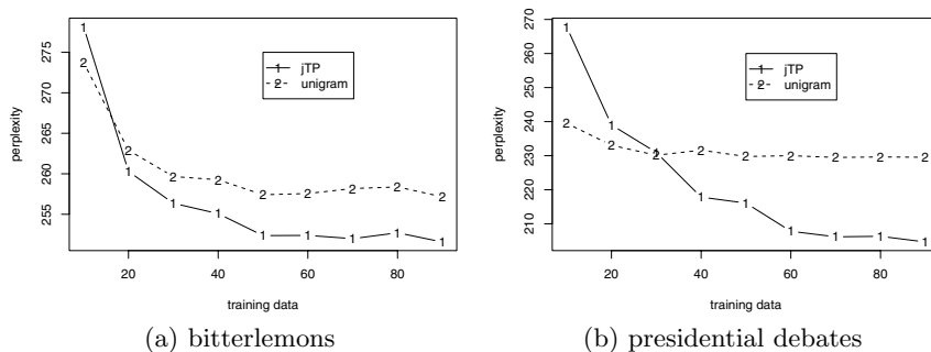
Fig. 8. The proposed joint topic and perspective model reduces perplexity on a held-out set
